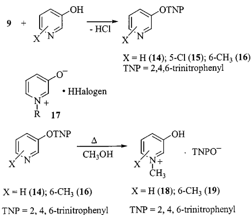
Scheme 5. Reactions between 3-hydroxypyridines and 9 and transformation of 14 and 16 in methanol
