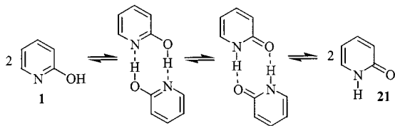
Scheme 10. Tautomerism of 2-hydroxypyridine by dimer formation
