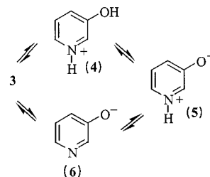
Scheme 2. Tautomerism of 3-hydroxypyridine
