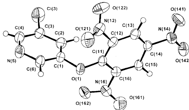
Figure 1. Perspective view and atom labelling of compound 15 ; displacement ellipsoids are drawn at the 50% probability level and H atoms are drawn as small circles of arbitrary radii
