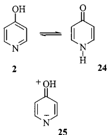
Scheme 11. Tautomerism of 4-hydroxypyridine
