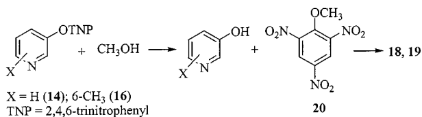
Scheme 6. Mechanism of the reaction between 14 (and 16 ) and methanol
