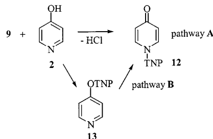
Scheme 4. Reaction pathways to compound 12
