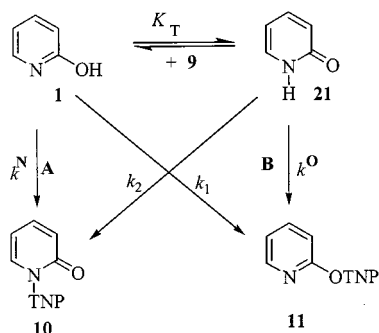
Scheme 8. Reaction pathways of 2-hydroxypyridine with 9
