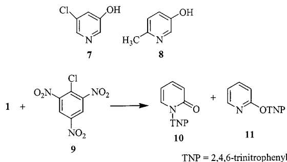
Scheme 3. Reactions between 2-hydroxypyridine ( 1 ) and 1-chloro-2,4,6-trinitrobenzene ( 9 )
